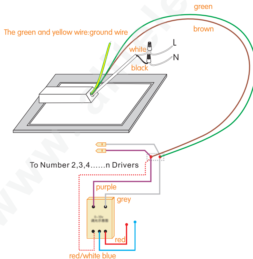
(2) 0-10V dimmable diagram
