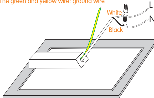
(1) Non-dimmable wiring diagram
