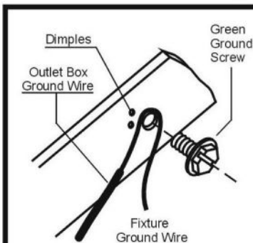
Fig. B Grounding Detail
