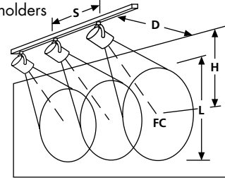
Figure 2 Multiple lampholders
