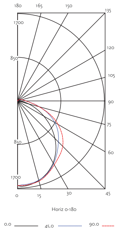
INDOOR CANDELA PLOT
